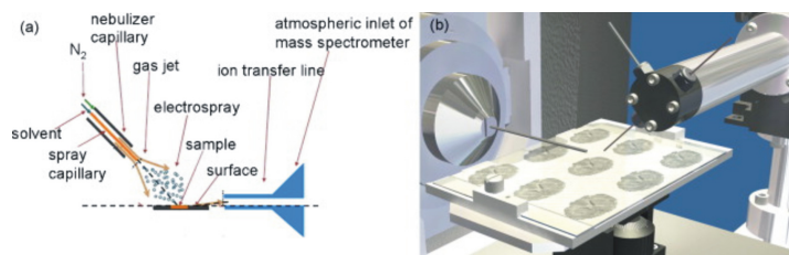
Figure 2.3 Desorption electrospray ionization. (A) Schematic representation of DESI desorption and ionization process; (B) brain tissue imaging analysis using DESI. Reprinted with permission from ref 79 . Copyright 2008 Elsevier.
