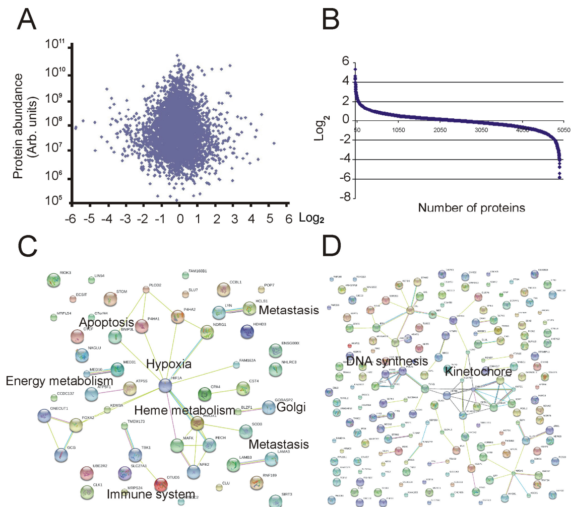
Figure 6.1 (A) Hypoxia-induced proteome changes in breast cancer. The x-axis represents the \log_2 change in protein expression, while the y-axis shows the peak area of peaks identified by mass spectrometric analysis. (B) The x-axis shows the number of quantified proteins, while the y-axis represents the \log_2 change in protein expression. (C) String analysis of up-regulated proteins 464 . (D) String analysis of down-regulated proteins.
