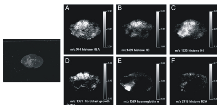
Figure 2.17 MALDI MS images of peptides distribution within an MCF-7 xenograft tissue section. Reprinted with permission from ref 35 . Copyright 2008 American Chemical Society.
